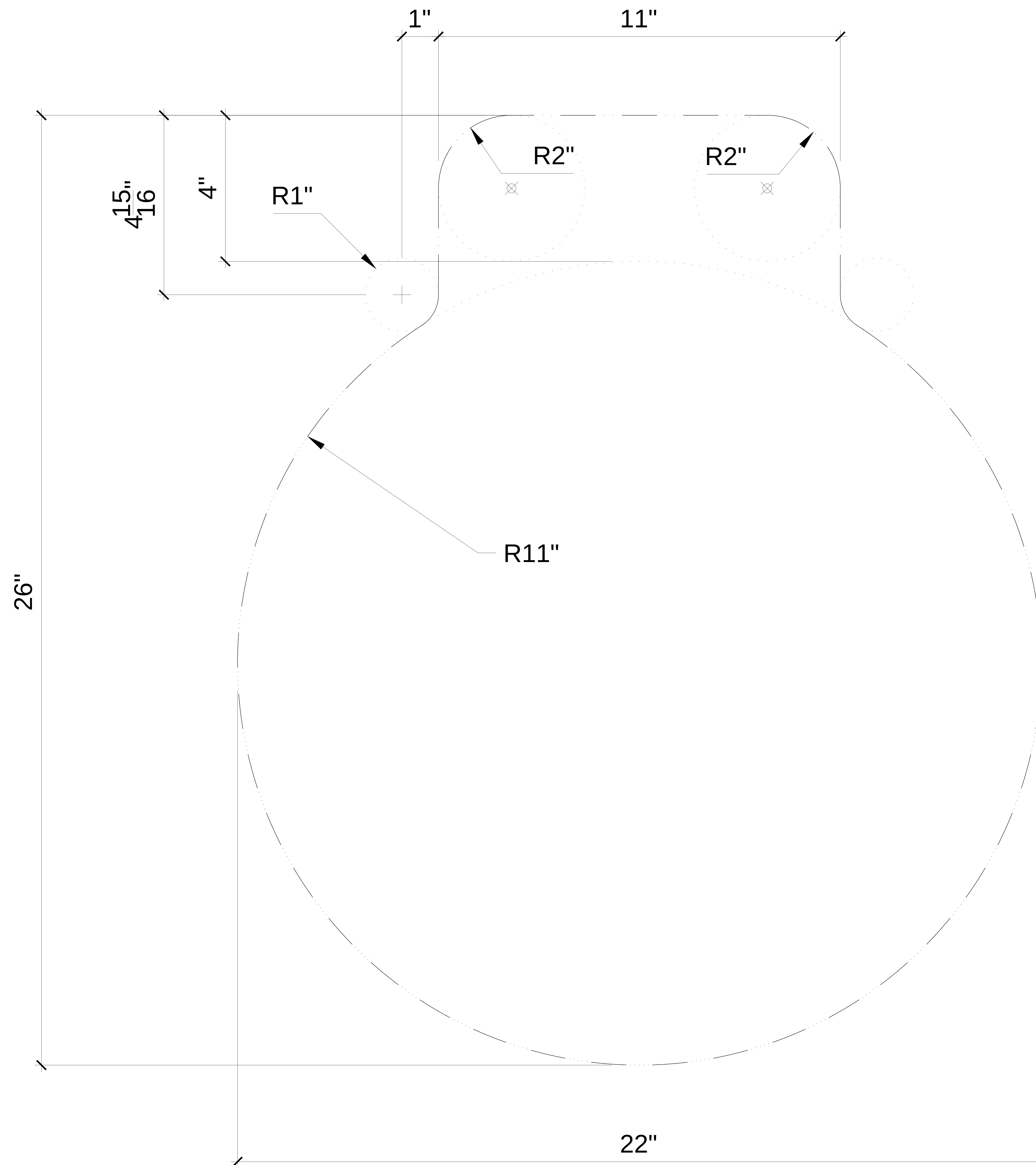
FIG. A - PLAN VIEW CUT-OUT
