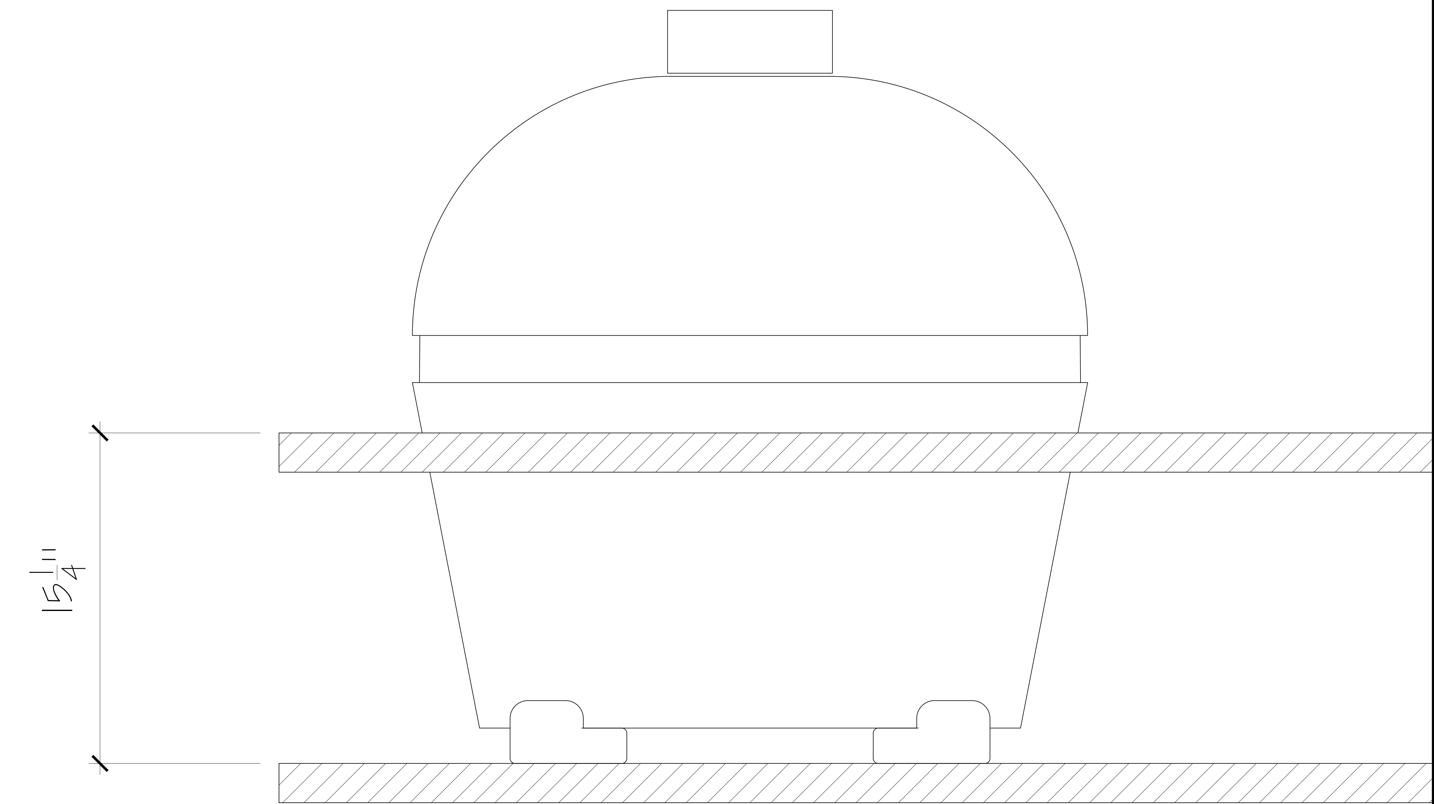
FIG. B - ELEVATION - HT. FROM TOP SURFACE TO SUPPORTING SHELF
