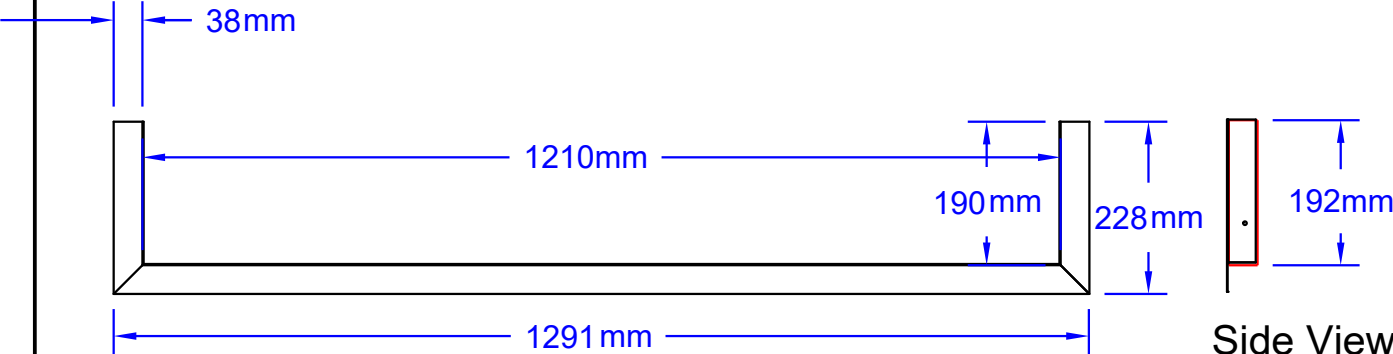
Front View
